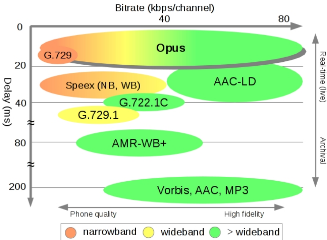
Bitrate/Latency Comparison
