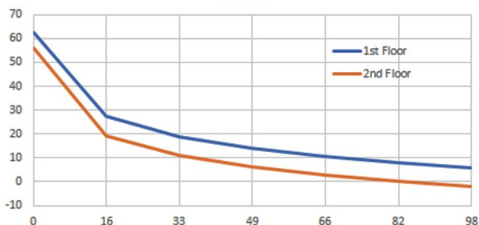
Smartphone Link Margin vs Range from WiFi Router
