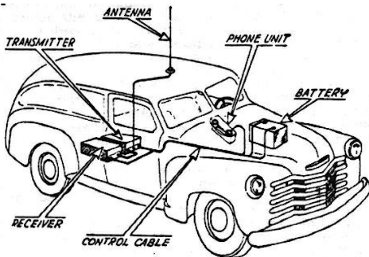
FIG. 4—Typical Mobile Installation
