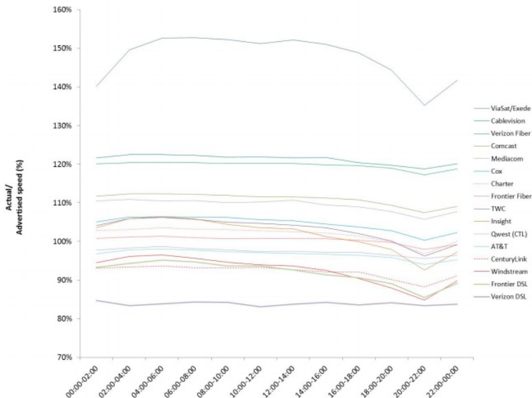
Chart 17: Hourly Sustained Download Speeds as a Percentage of Advertised, by Provider—September 2013 Test Data
