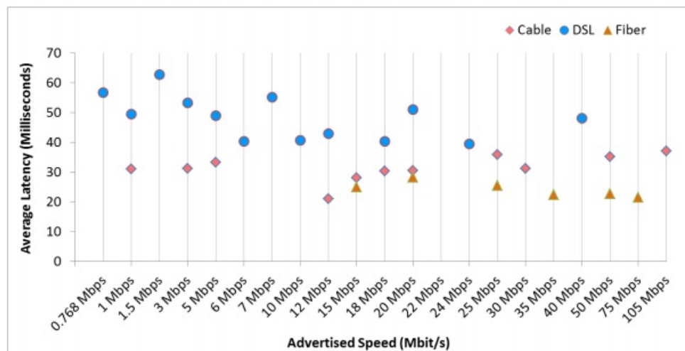
Chart 14: Average Peak Period Latency in Milliseconds, by Technology—September 2013 Test Data
