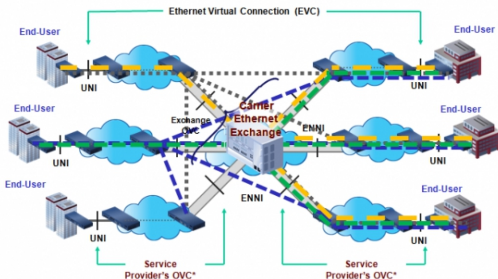
Carrier Ethernet Exchange Model, презентация MEF Global Interconnect
